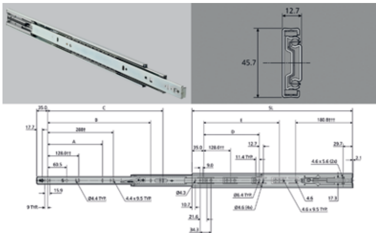
Accuride geleider type 3832 B
